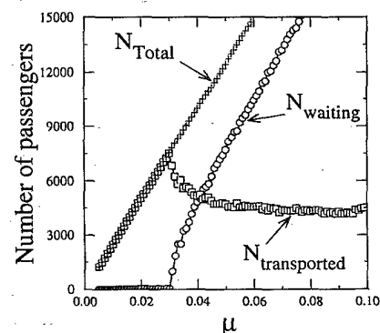
FIG. 2. Accumulated population density after 5000 time steps. Above \mu \approx 0.03 the transport is not efficient anymore.
