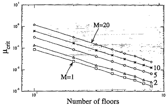
FIG. 3. Critical values of \mu as functions of the number of floors and number of elevators. As seen in Fig. 2, beyond \mu_{\text{crit}} the transport is not efficient anymore. The characteristic exponent underlying all curves is \mu \approx N^{-1.88} .
